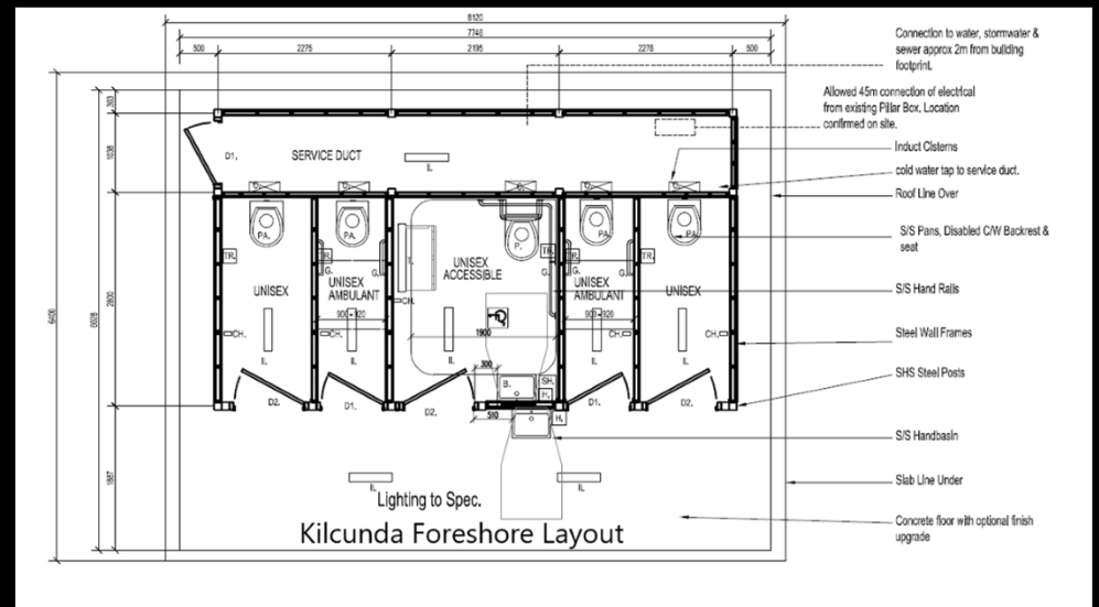
Kilcunda Foreshore Toilet layout plan
