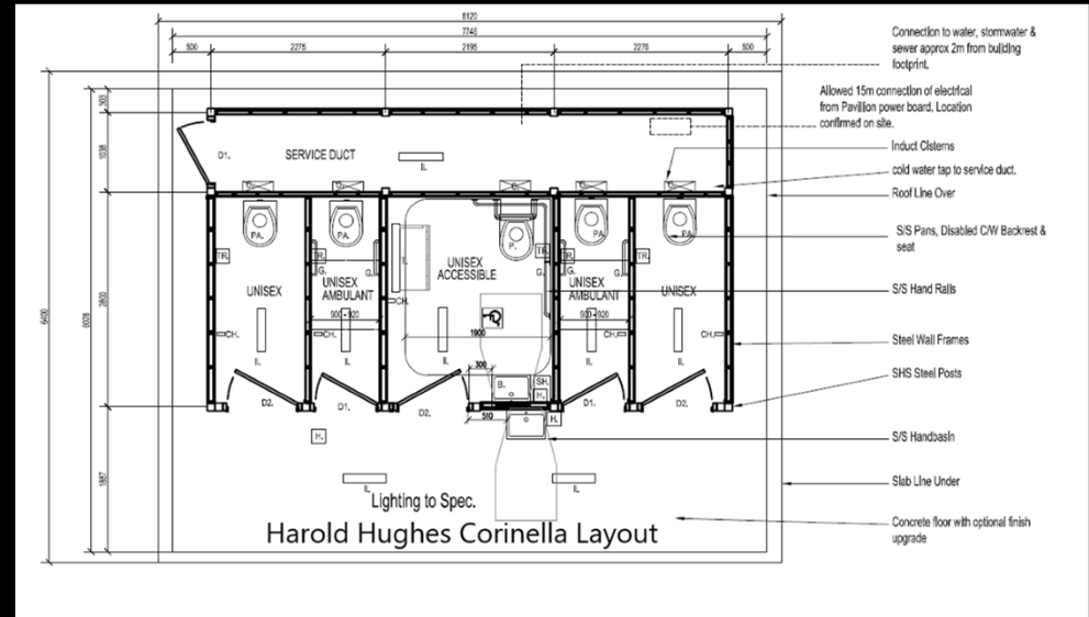
Harold Hughes Toilet layout plan
